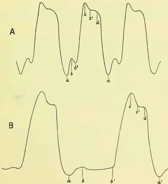
FIG. 39. CURVES OF ENDOCARDIAC PRESSURE. FROM LEFT VENTRICLE OF DOG.
